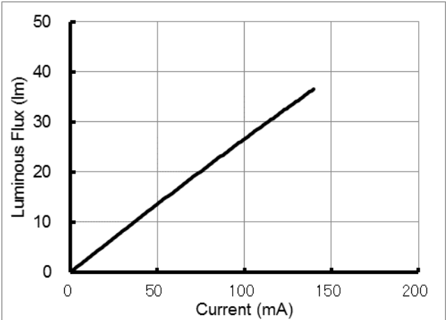
●Forward current vs. Total luminous flux [Ta=25°C]
