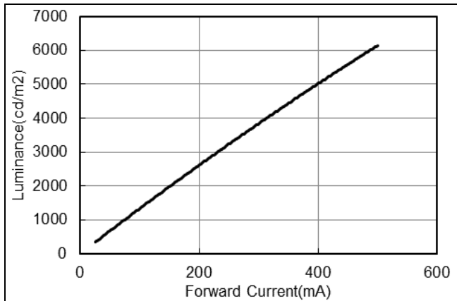
● Forward current vs. Luminance [ T_a=25^\circ\text{C} ]
