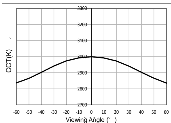
● Angular dependence in correlated color temperature [ I_f=210\text{mA} T_a=25^\circ\text{C} ]
