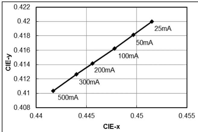
● Forward current vs. Chromaticity [ T_a=25^\circ\text{C} ]
