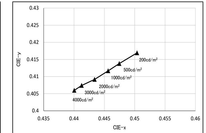
● Luminance vs. Chromaticity [ T_a=25^\circ\text{C} ]
