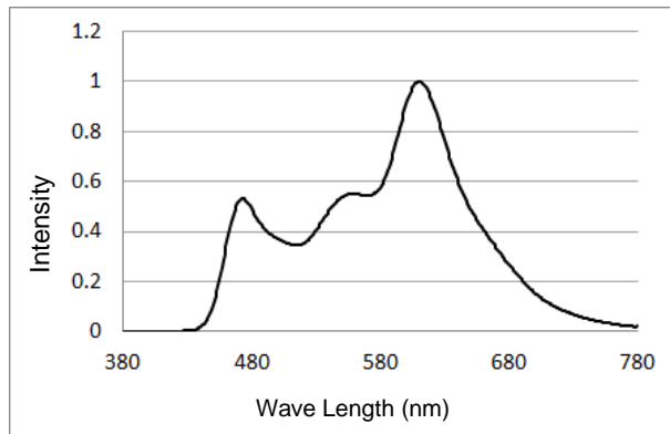
● Spectral distribution [ I_f=210\text{mA} T_a=25^\circ\text{C} ]
